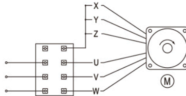
三相AC380V接线图 Three-phase AC380V Wiring Diagrams
