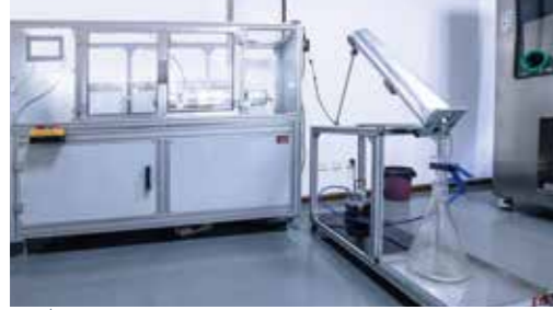
储气罐清洁度萃取设备 / Air Reservoir Cleanliness Extraction Equipment
